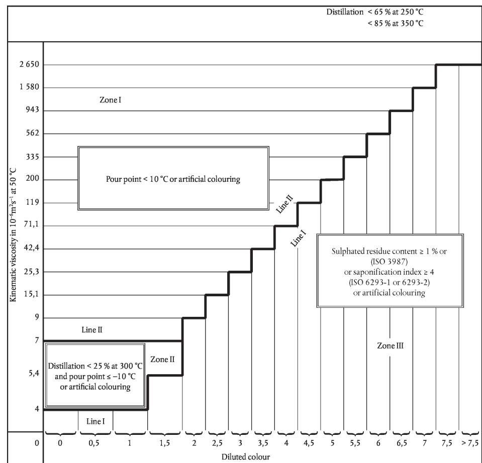
Characteristics of lubricating and other oils
