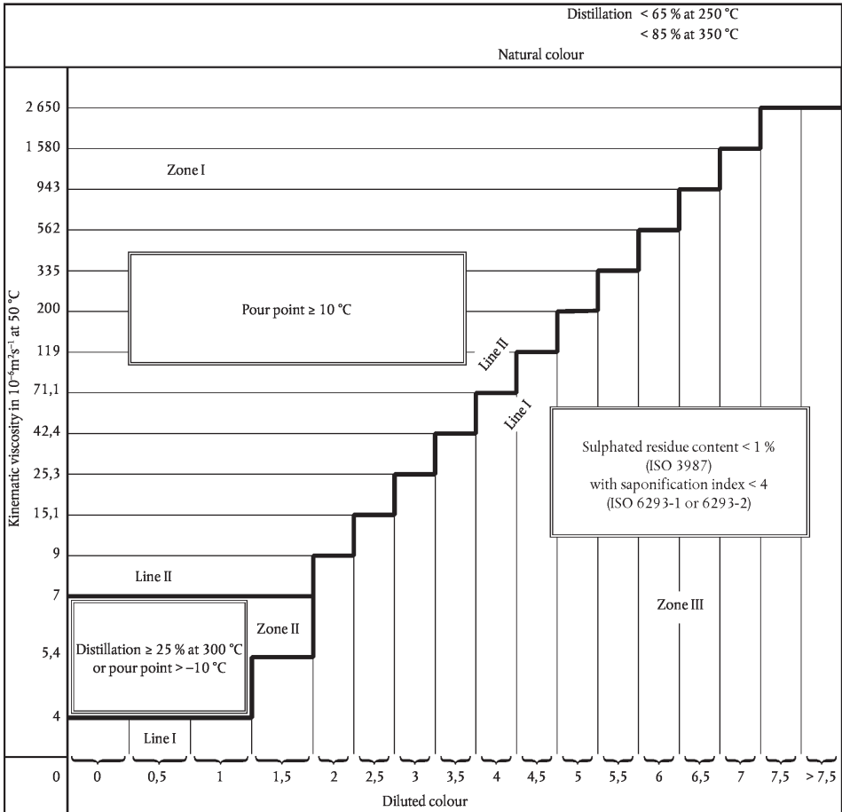
Characteristics of fuel oils
